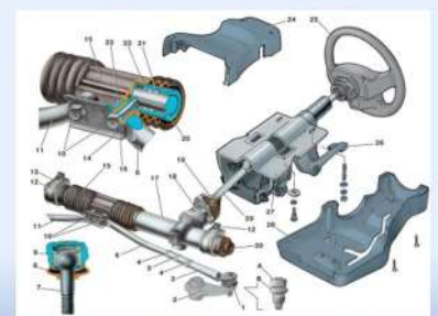
STEERING SYSTEM
